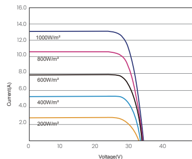
昊宇光伏I-V曲线图(425W)
