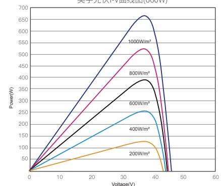
昊宇光伏I-V曲线图(660W)
