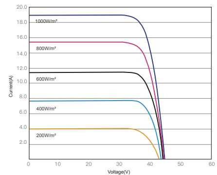
昊宇光伏I-V曲线图(660W)
