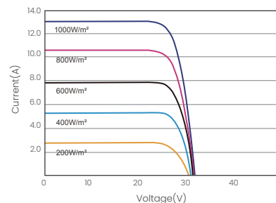
昊宇光伏I-V曲线图(410W)
