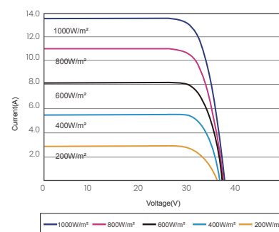
昊宇光伏I-V曲线图(400W)
