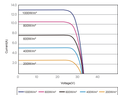
昊宇光伏I-V曲线图(410W)
