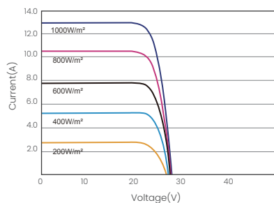
昊宇光伏I-V曲线图(360W)
