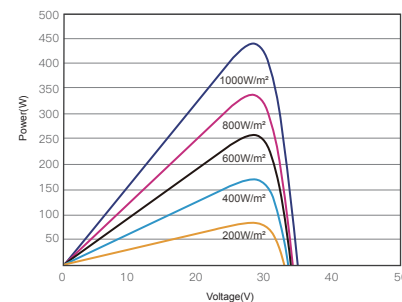
昊宇光伏P-V曲线图(440W)
