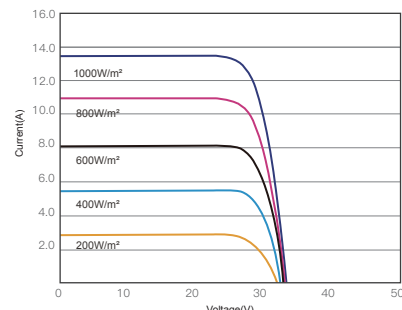
昊宇光伏I-V曲线图(440W)
