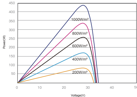
昊宇光伏P-V曲线图(440W)
