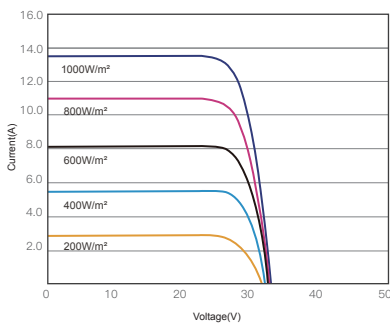
昊宇光伏I-V曲线图(440W)
