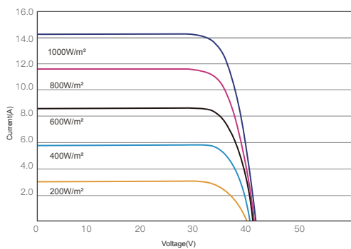
昊宇光伏I-V曲线图(580W)
