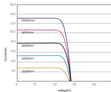
昊宇光伏I-V曲线图(370W)
