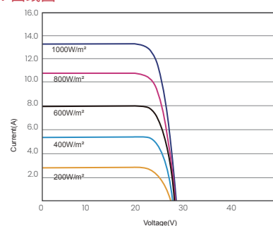
昊宇光伏I-V曲线图(380W)
